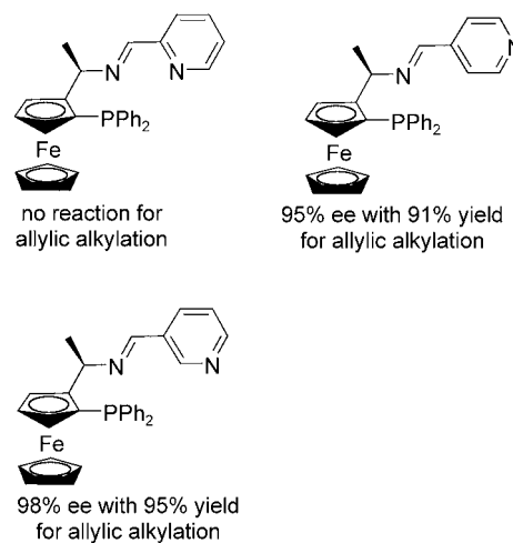
Figure 1. Influence of the pyridine N atom on Pd-catalyzed asymmetric allylic alkylation.
