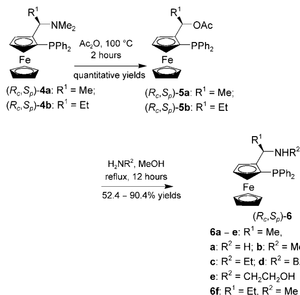
Scheme 1. Synthesis of ferrocenylphosphine-amines ( R c S p )- 6a–f .
