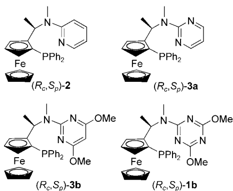
Figure 3. Structures of ligands (R_c,S_p) -1b, (R_c,S_p) -2 and (R_c,S_p) -3.
