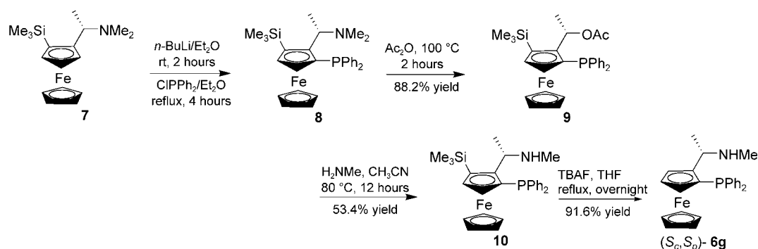
Scheme 2. Synthesis of ferrocenylphosphine-amines (S_c,S_p) -6g.
