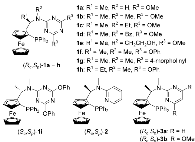
Figure 2. Structures of ferrocenylphosphine-heterocycle ligands 1 , 2 and 3 .
