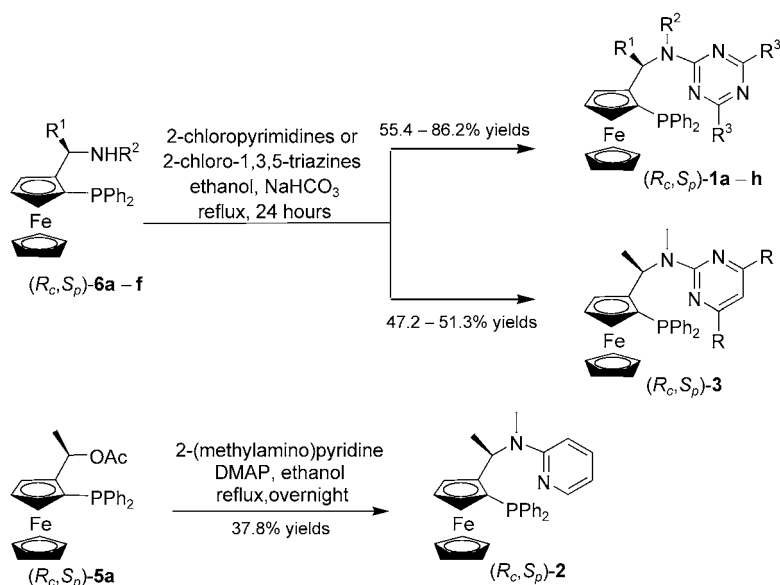
Scheme 3. Synthesis of ferrocene-based phosphine-heterocycle ligands 1 , 2 and 3 .
